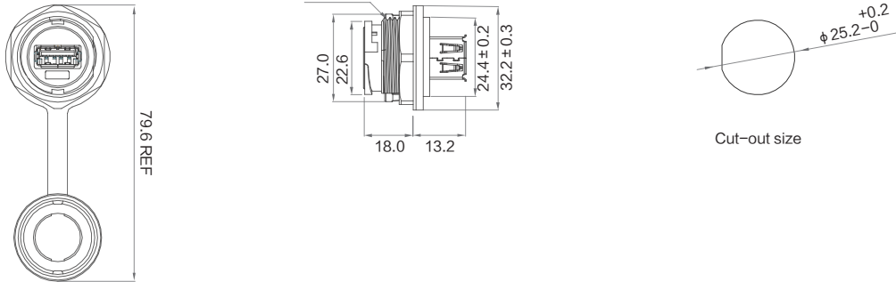
Single hole straight receptacle
