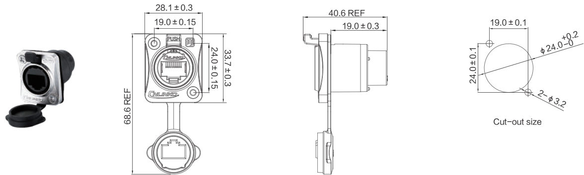
Metal Square Receptacle YT-RJ45-JSX-17-001
