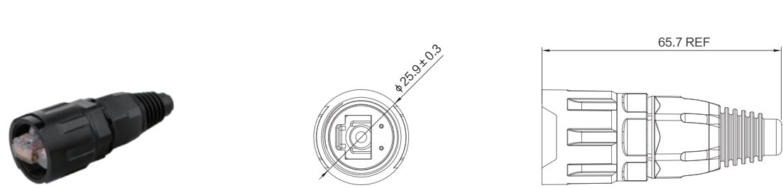
Plastic Circular Connector YT-RJ45-CPE-29-001
