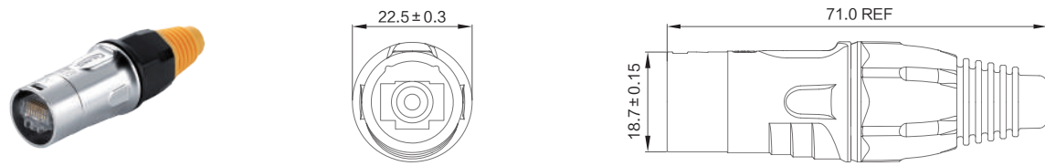
Metal Square Receptacle YT-RJ45-JSX-16-001
