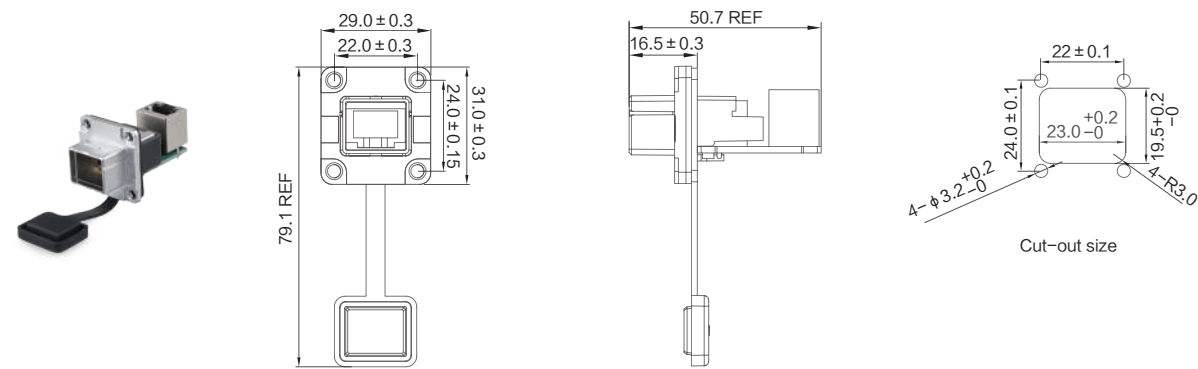
Square Receptacle YT-RJ45-JSX-08-001
