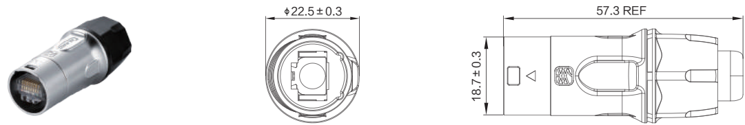
Metal Circularplug Connector YT-RJ45-CPE-10-001/2
