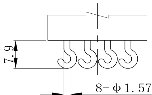
Pin Form "4"
