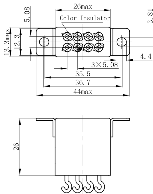
Mounting Code "8"
