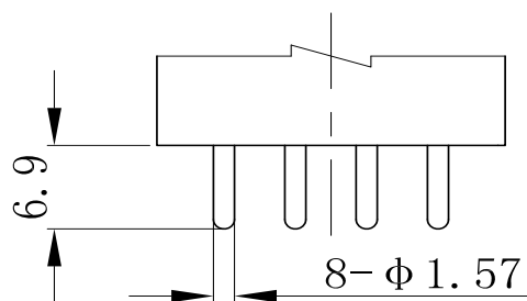
Pin Form "1"
