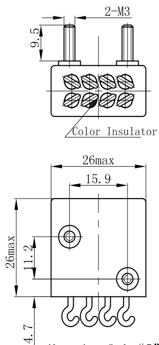
Mounting Code "5"
