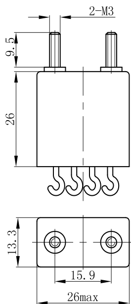
Mounting Code "4"
