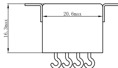
Mounting Code "8"
