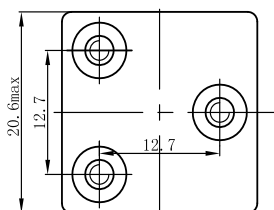
Mounting Code "4"
