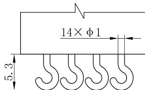
Pin Form "4"
