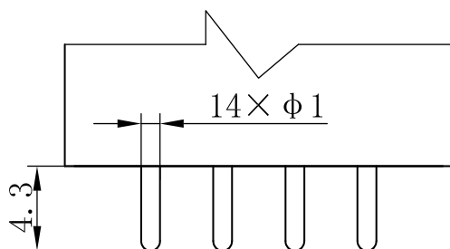
Pin Form "1"
