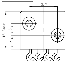
Mounting Code "5"
