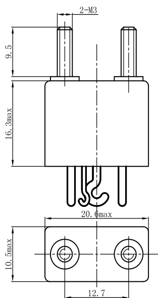
Mounting Code "4"
