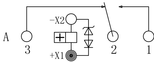
JQC-1110M
