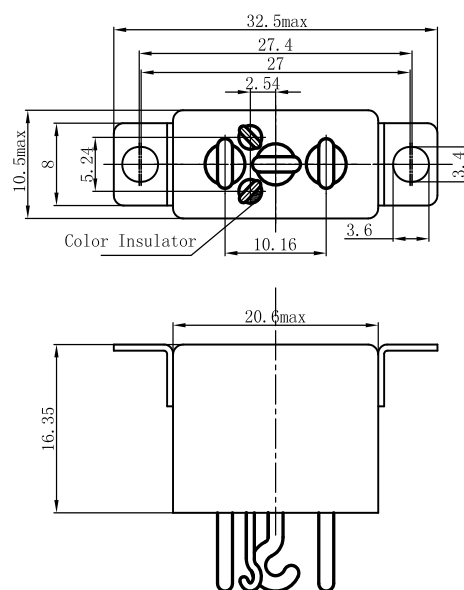
Mounting Code "8"
