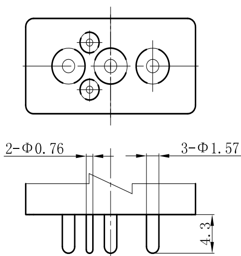
Pin Form "1"
