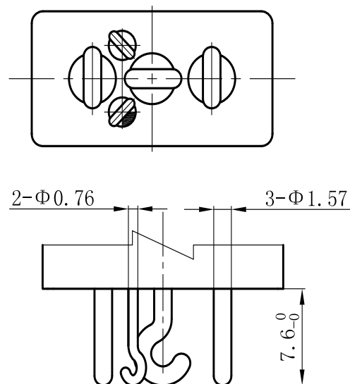
Pin Form "4"
