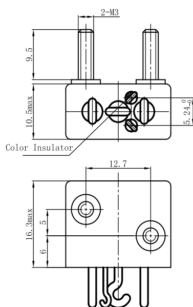
Mounting Code "5"
