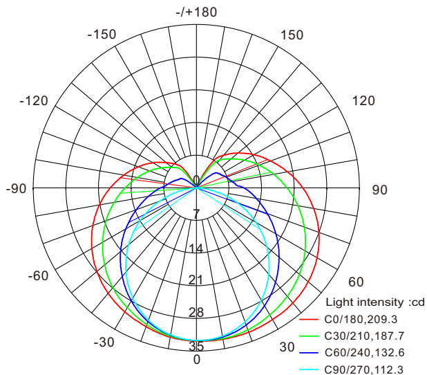
Light distribution curve
