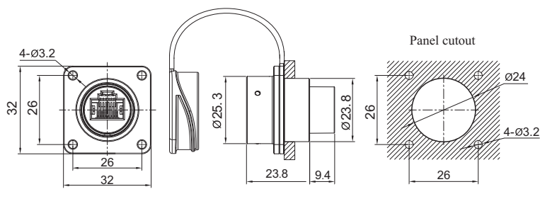
RJ45 Square flange receptacle Mate with SF2410
