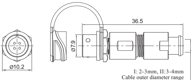
In-line cable connector Mate with SF610S
