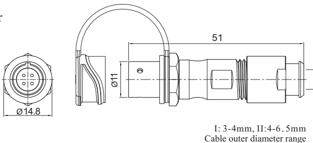
In-line cable connector Mate with SF1010S
