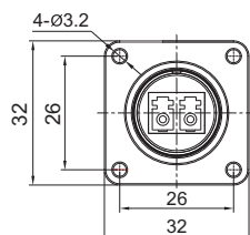
Square flange receptacle with LC adapter Mate with SF2410
