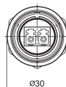
Rear-nut mount receptacle with LC adapter Mate with SF2410
