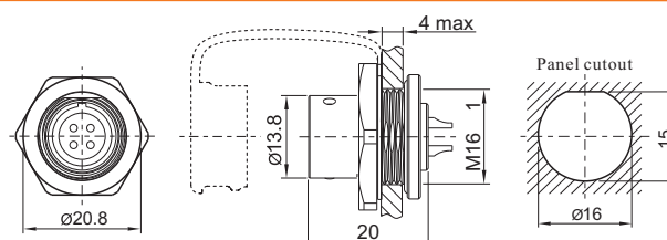
Front-nut mount Mate with SF1210, SF1214
